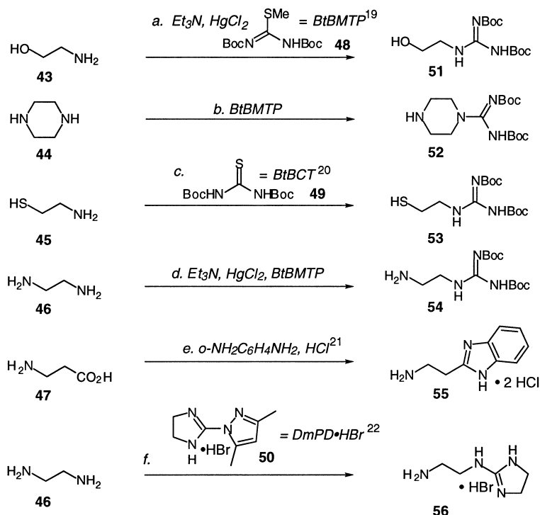
Scheme 3. Synthesis of guanidine derivatives 51–56 . Reagents and conditions: (a) 1.0 equiv of Bt BMTP, 2.0 equiv of \text{Et}_3\text{N} , 1.0 equiv of \text{HgCl}_2 , DMF, 25 °C, 4 h, 98%; (b) 1.0 equiv of Bt BMTP, DMF, 25 °C, 14 h, 95%; (c) 1.0 equiv of Bt BCT, 2.0 equiv of \text{Et}_3\text{N} , DMF, 25 °C, 14 h, 60%; (d) 0.2 equiv of Bt BMTP, 0.4 equiv of \text{Et}_3\text{N} , 0.2 equiv of \text{HgCl}_2 , DMF, 25 °C, 4 h, 51%; (e) 0.66 equiv of o - \text{NH}_2\text{C}_6\text{H}_4\text{NH}_2 , 5.5 N aq HCl, reflux, 24 h, 73%; (f) 1.0 equiv of DmPD-HBr, i -Pr 2 NEt, DMF, 25 °C, 11 h, 51%. Boc = tert -butoxycarbonyl; Bt BCT = N,N' -bis( tert -butoxycarbonyl)thiourea; Bt BMTP = 1,3-bis( tert -butoxycarbonyl)-2-methyl-2-thiopseudourea; DmPD-HBr = 2-(3,5-dimethylpyrazolyl)-4,5-dehydroimidazole hydrobromide.
