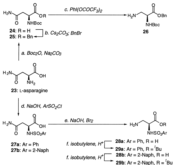
Scheme 1. Synthesis of amino esters 26 , 29a , and 29b . Reagents and conditions: (a) 1.1 equiv of Boc 2 O, 1.0 equiv of Na 2 CO 3 , 1,4-dioxane, H 2 O, 25 °C, 88%; (b. i.) 20% aq solution of Cs 2 CO 3 , H 2 O:MeOH (1:2.5), 25 °C, 4 h, 100%; (ii) 1.1 equiv of BnBr, DMF, 25 °C, 14 h, 88%; (c) 1.5 equiv of PhI(OCOCF 3 ) 2 , DMF:H 2 O (1:1), 2.0 equiv of pyridine, 25 °C, 3.5 h, 41%; (d) 1.1 equiv of ArSO 2 Cl, 2.25 equiv of NaOH, dioxane:H 2 O (1:2), 0→25 °C, 3 h, [71% for 27a , 66% for 27b ]; (e) 1.3 equiv of Br 2 , 9.2 equiv of NaOH, H 2 O, 0→90 °C, [75% for 28a , 81% for 28b ]; (f) isobutylamine, 2.8 equiv of concd H 2 SO 4 , DME, −78→25 °C, 48 h, [55% for 29a , 51% for 29b ]. DME = dimethoxyethane; DMF = dimethylformamide; 2-Naph = 2-naphthyl.
