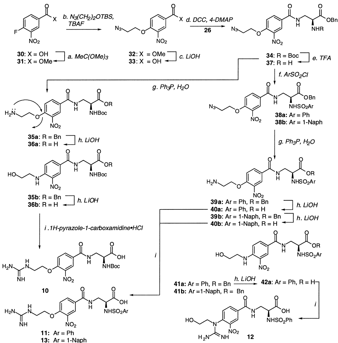
Scheme 2. Synthesis of compounds 10–13 . Reagents and conditions: (a) 5.0 equiv of MeC(OMe) 3 , PhMe, 80 °C, 8 h, 98%; (b) 1.1 equiv of N 3 (CH 2 ) 2 OTBS, 0.1 equiv of TBAF, 4 Å MS, DMF, 25 °C, 4 h, 73%; (c) 2.0 equiv of LiOH·H 2 O, dioxane:H 2 O (3:1), 25 °C, 4 h, 99%; (d) 1.0 equiv of DCC, 0.2 equiv of 4-DMAP, CH 2 Cl 2 , 25 °C, 4 h, 82%; (e) 50% TFA in CH 2 Cl 2 , 25 °C, 2 h, 84%; (f) 1.1 equiv of PhSO 2 Cl or 1-NaphSO 2 Cl, 1.3 equiv of i -Pr 2 NEt, CH 2 Cl 2 , 25 °C, 4 h, 38a (78%), or 38b (57%); (g) 2.0 equiv of Ph 3 P, 44 equiv of H 2 O, THF, 25 °C, 12 h, 80%, ca. 1:1 of 35a:35b ; 80%, ca. 1:1 of 39a:41a ; 81%, ca. 1:1 of 39b:41b ; (h) 2.0 equiv of LiOH·H 2 O, THF:H 2 O (3:1), 25 °C, 4 h, 93–99% for 36ab , 40ab , 42a ; (i) 1.1 equiv of 1 H -pyrazole-1-carboxamide·HCl, 1.1 equiv of i -Pr 2 NEt, DMF, 25 °C, 16 h, 13–15% for 10 , 11 , 13 ; 50 °C, 16 h, 5% for 12 , after RP-HPLC. TFA = trifluoroacetic acid; TBAF = tetra- n -butylammonium fluoride; DCC = 1,3-dicyclohexylcarbodiimide.
