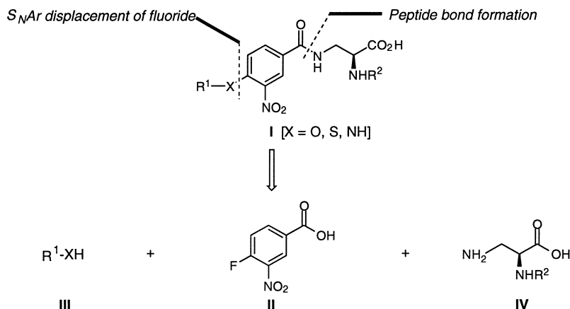
Figure 4. General structures of nitroaryl ether peptide mimetics and retrosynthetic analysis.
