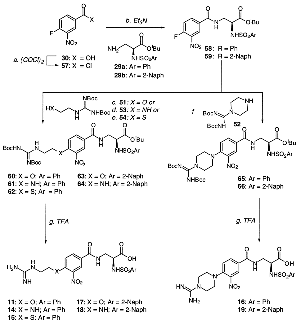
Scheme 4. Synthesis of compounds 11 and 14–19 . Reagents and conditions: (a) 1.2 equiv of (\text{COCl})_2 , PhH, DMF, 0^\circ\text{C} , 6 h, 99%; (b) 1.0 equiv of 29a or 29b , 1.2 equiv of \text{Et}_3\text{N} , \text{CH}_2\text{Cl}_2 , 0^\circ\text{C} , 2 h, 58 (98%), or 59 (96%); (c) for 60 : 2.2 equiv of NaH, 2.2 equiv of 51 , DMF, 25^\circ\text{C} , 8 h, 66%; for 63 : 4.0 equiv of NaH, 1.2 equiv of 51 , DMF, 25^\circ\text{C} , 4 h, 69%; (d) 1.1 equiv of 53 , DMF, 25^\circ\text{C} , 4 h, 73%; for 64 : 1.9 equiv of 53 , NMP, 25^\circ\text{C} , 99%; (e) for 65 : 2.2 equiv of NaH, 2.5 equiv of 54 , DMF, 25^\circ\text{C} , 12 h, 23%; (f) 1.1 equiv of 52 , DMF, 25^\circ\text{C} , 6 h, 83%; for 66 : 2.0 equiv of 52 , DMF, 25^\circ\text{C} , 20 h, 99%; (g) 50% TFA in \text{CH}_2\text{Cl}_2 , 25^\circ\text{C} , 30 min, 90–99% for 11 , 14–19 after RP-HPLC. Boc = tert -butoxycarbonyl; TFA = trifluoroacetic acid; NMP = N -methyl-2-pyrrolidinone; DMF = dimethylformamide.
