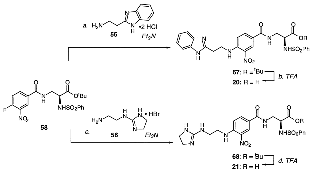
Scheme 5. Synthesis of compounds 20 and 21 . Reagents and conditions: (a) 1.0 equiv of 55 , 2.2 equiv of Et 3 N, DMF, 25 °C, 16 h, 92%; (b) 50% TFA in CH 2 Cl 2 , 25 °C, 4 h, 97%; (c) 1.0 equiv of 56 , 2.2 equiv of Et 3 N, DMF, 12 h, 110% (crude yield); (d) 50% TFA in CH 2 Cl 2 , 25 °C, 4 h, 83% after RP-HPLC; TFA = trifluoroacetic acid; DMF = dimethylformamide.
