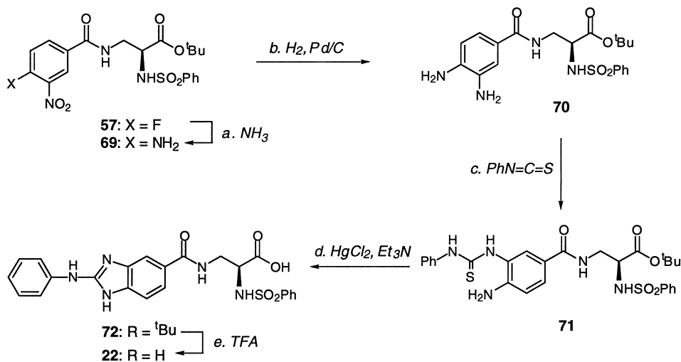
Scheme 6. Synthesis of compound 22 . Reagents and conditions: (a) NH 3 , DMF, 25 °C, 5 h, 93%; (b) 10% Pd/C, H 2 , MeOH, 25 °C, 8 h, 90%; (c) 1.1 equiv of PhNCS, EtOH, 14 h, 69%; (d) 1.0 equiv of HgCl 2 , 1.0 equiv of Et 3 N, DMF, 4 h, 81%; (e) 50% TFA in CH 2 Cl 2 , 30 min, 88% yield, after RP-HPLC. TFA = trifluoroacetic acid; DMF = dimethylformamide.
