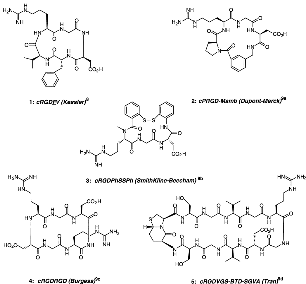
Figure 1. Selected structures of \alpha_v\beta_3 antagonists.
