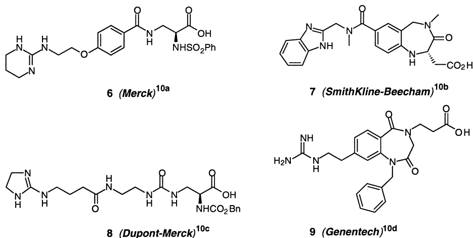
Figure 2. Selected nonpeptide mimetics with high affinity for \alpha_v\beta_3 .
